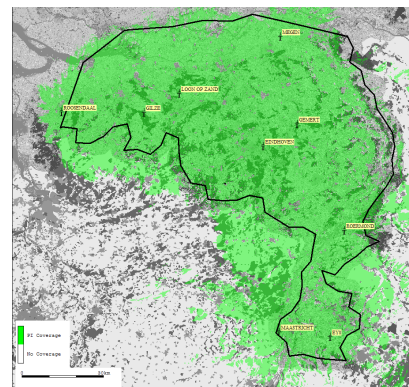
Picture: Portable Indoor coverage (95% location probability) for allotment 7A
